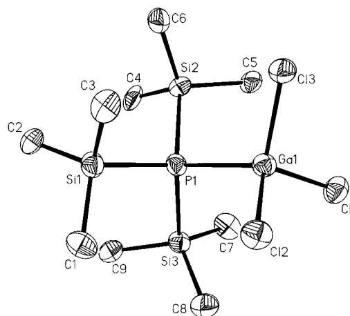
Figure 3. ORTEP diagram (35% probability ellipsoids) showing the solid-state structure and atom-numbering scheme of 1. The solvent structure and hydrogen atoms are omitted for clarity.
