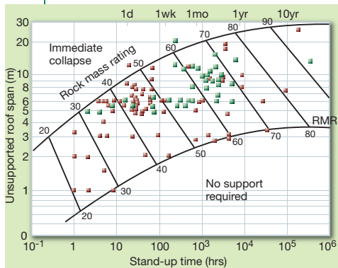
Above: Fig 4 - Stand up time as a function of RMR and unsupported tunnel span (Bieniawski, 1989). Red squares represent tunnelling cases, green squares are mining data
