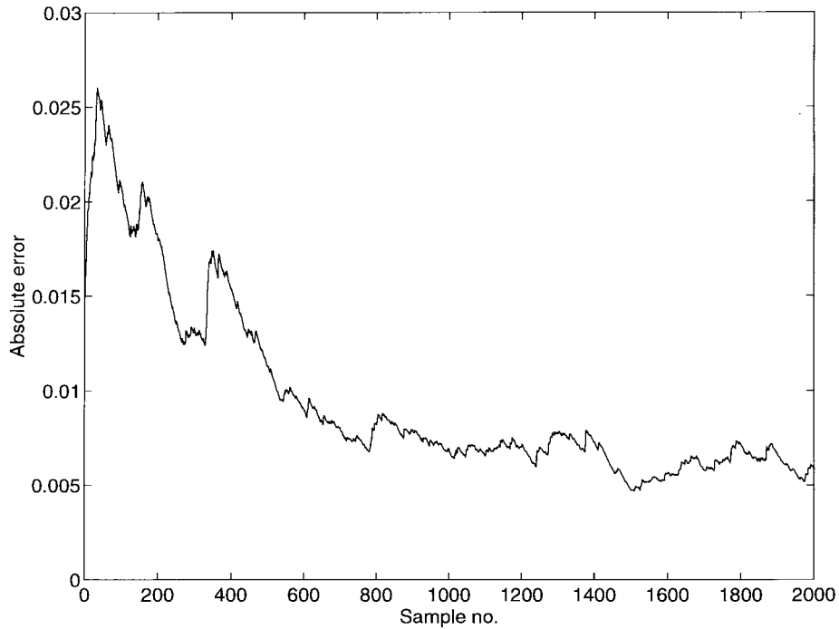
Fig. 7. Time history of absolute error during on-line training.
