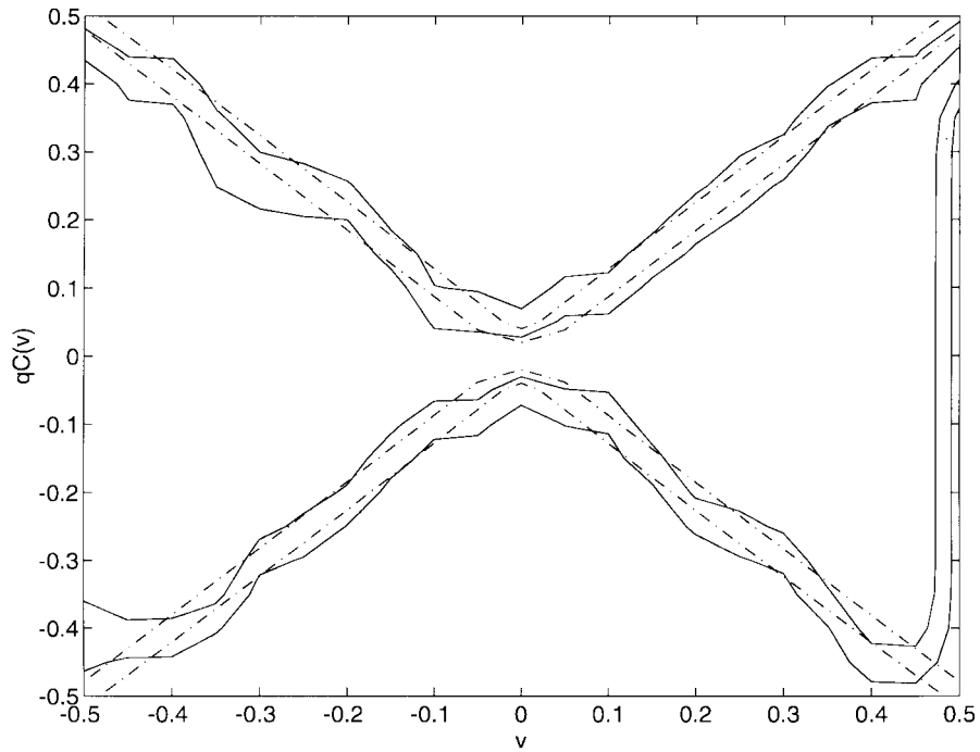
Fig. 4. Estimated and theoretical conditional quantiles.
