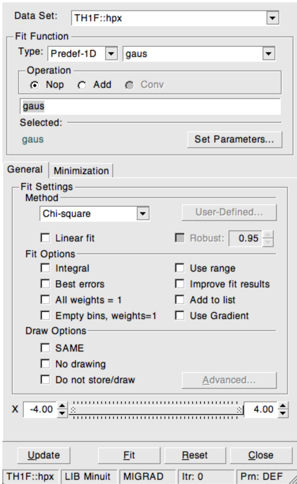
Figure 2.5: Fit Panel.
