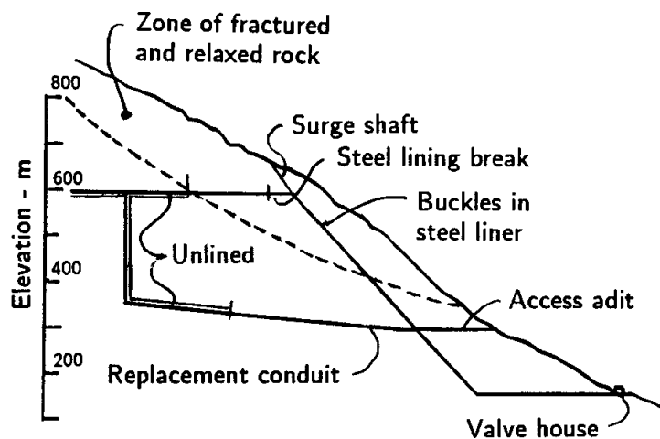
Figure 2.3 : Cross-section through a section of the Wahleach power tunnel showing the original tunnel alignment and the location of the replacement conduit. The dashed line is the approximate location of a gradational boundary between loosened, fractured and weathered rock and more intact rock. Down-slope movement currently being monitored is well above this boundary.
