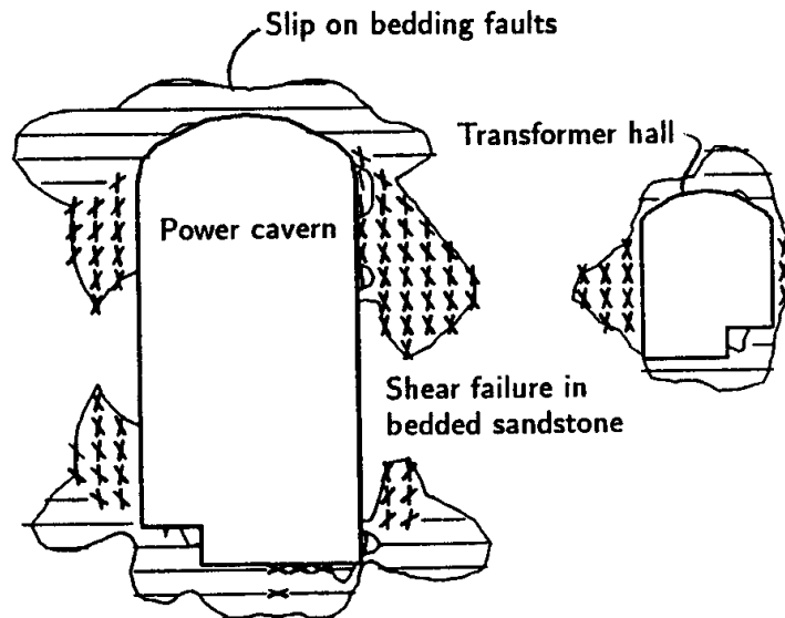
Figure 2.5 : Predicted zones of over-stress along faults and in bedded sandstone surrounding the power cavern and transformer hall of the Mingtan Project.
