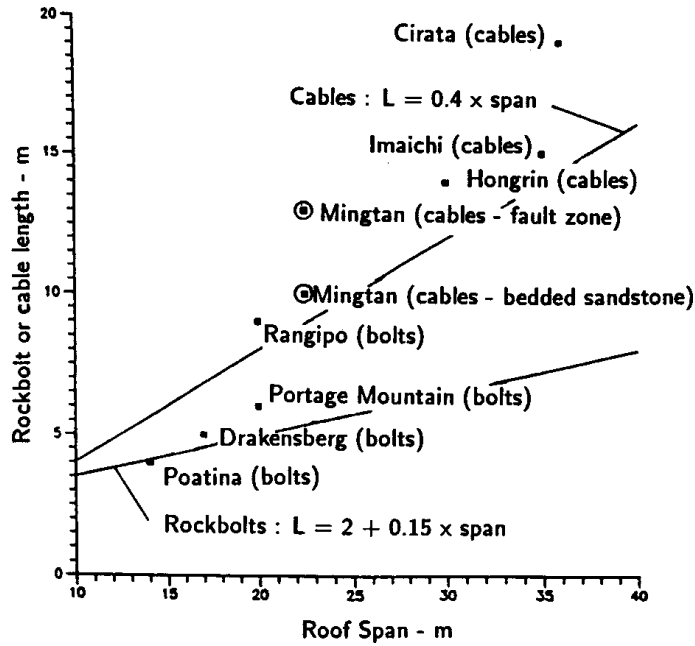
Figure 2.6 : Lengths of rockbolts and cables used for roof support in some large caverns in weak rock. Equations defining trend lines were suggested by Barton (1989).
