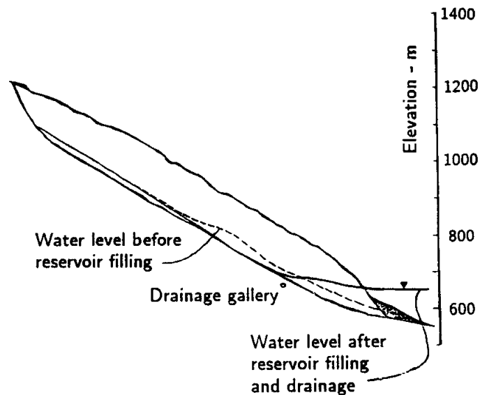
Figure 2.1 : Section through Dutchman's Ridge showing potential slide surface and water levels before and after drainage.
