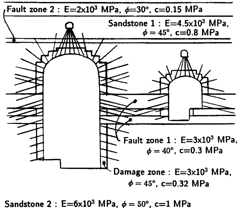
Figure 2.8 : Layout of cables used to support the rock surrounding the power cavern and the transformer hall in the Mingtan pumped storage project. The location and properties of the rock units represent those used in the numerical analysis of failure, deformation and cable loading in a typical vertical section.
