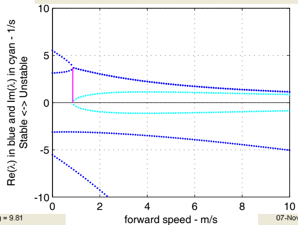
Figure 6.1: A bicycle of common construction but with the gyroscopic terms eliminated. The model is based on the benchmark bicycle [6] where the only change that has been made is to eliminate the spin angular momentum of the wheels. This bicycle is unstable at all forward speeds.
