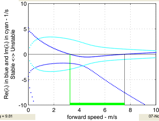
Figure 6.6: The model is based on the theoretical two-mass-skate (TMS) model from Chapter 7, but with slightly negative gyroscopic action (e.g., by counter-spinning wheels) and where the center of mass of the front fork has been lowered to 0.2 m. This bicycle has a large stable forward speed range.
