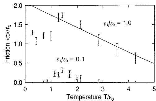
FIG. 5. Friction vs temperature data in normalized units for the case of strong ( \epsilon_1/\epsilon_0=1.0 ) and weak ( \epsilon_1/\epsilon_0=0.1 ) interfacial interactions at a sliding speed, v=20 m/s. The solid line represents a fit to the data using a thermal activation model (Ref. 35).
