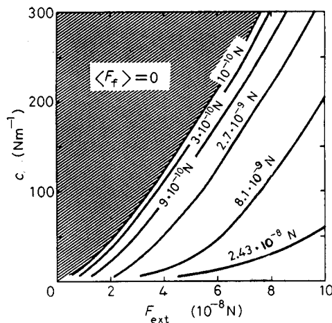
FIG. 4. Contour plot of the average friction force ( \langle F_f \rangle ) per atom as a function of the load F_{\text{ext}} and the horizontal spring constant c (for monoatomic Pd tip on graphite) (Refs. 31 and 32).
