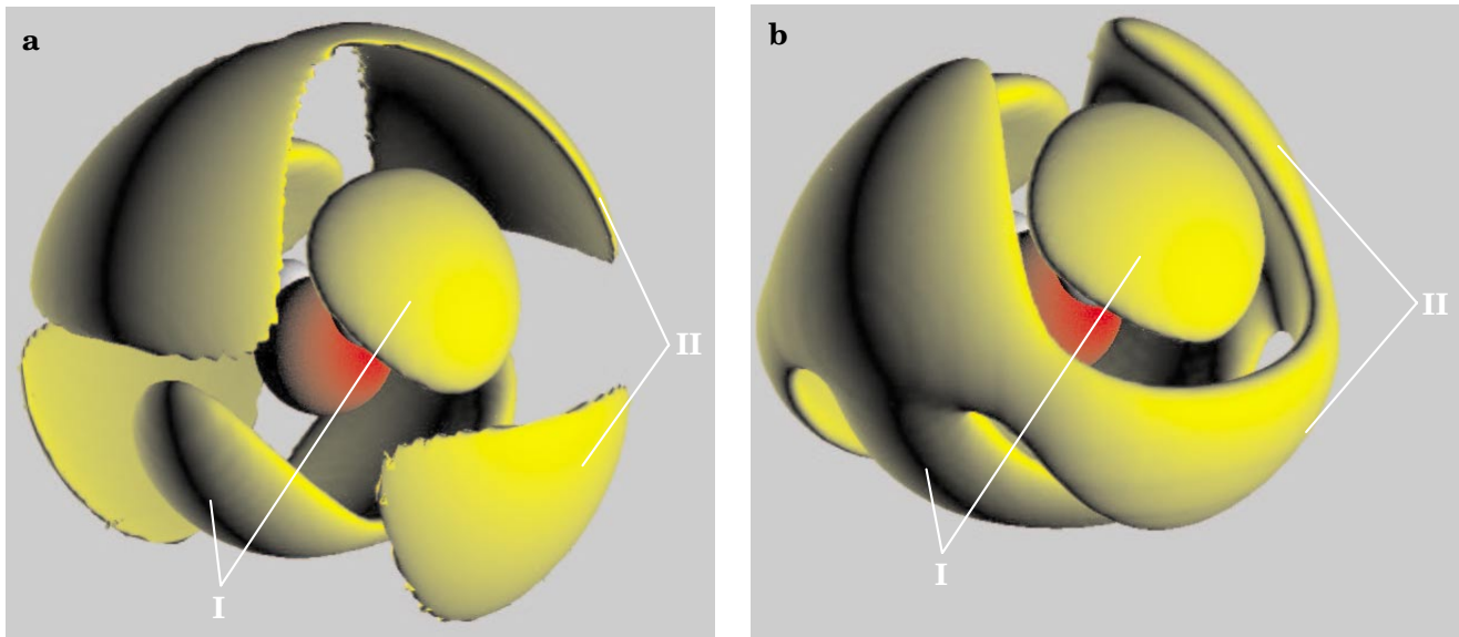
Figure 6. Contours of constant density around a central water molecule at 268 K for (a) low-density liquid water (LDL) and (b) high-density liquid water (HDL). The oxygen atom is shown in red; hydrogen atoms are partially visible as white lobes attached to the oxygen. The contours were calculated by a computer simulation that is constrained to reproduce the experimentally determined parameters (namely, the OO, OH, and HH structure factors measured by neutron diffraction 18 ). The contour levels have been set at 1.75 and 1.61 times the bulk density for LDL and HDL, respectively, so that the plotted surfaces enclose 25% of the water molecules in the range of 0.2–0.5 nm. Pronounced lobes (denoted I) are observed opposite each of the central molecule's OH vectors and in a broad band of density at right angles to those underneath the central molecule; these lobes correspond to the first shell of approximately tetrahedrally bonded molecules. A second shell, labeled II, is in antiphase with the first shell, and collapses in going from LDL to HDL. This collapse is the primary signature of the structural transformation that occurs as the density increases. (Courtesy of A. K. Soper and M. A. Ricci.)
