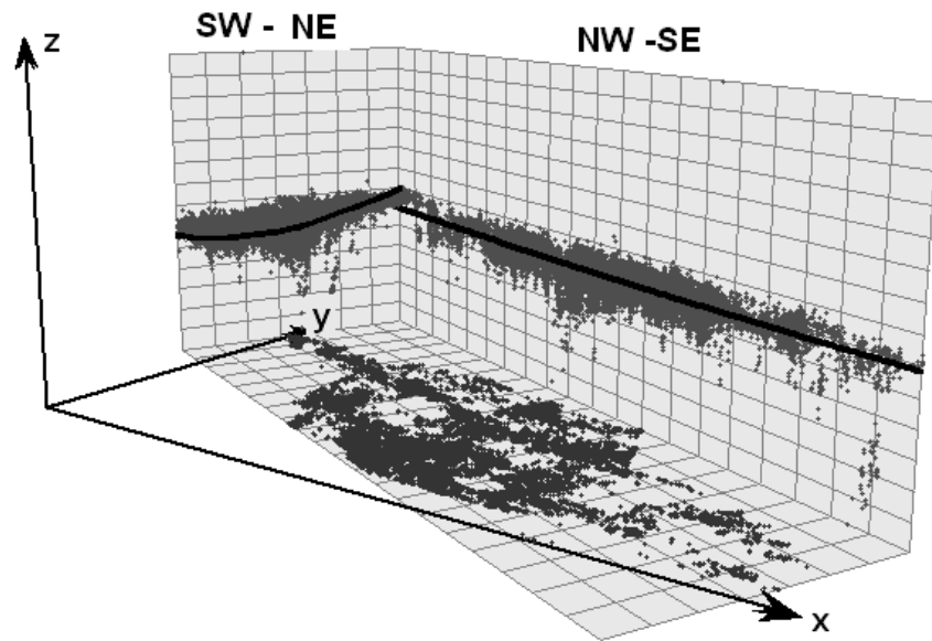
Fig.4.3. Trend analysis for directions SW-NE and NW-SE
