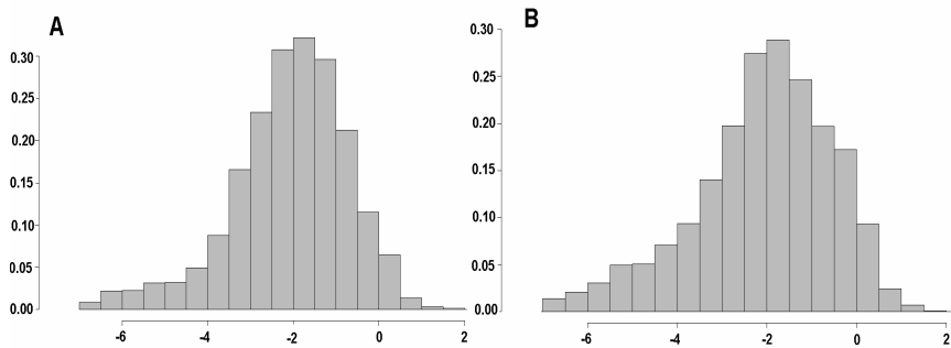
Fig.4.5. Histograms of average annual motion rate for faults with meridional strikes (A – upthrown blocks, B – downthrown blocks)
