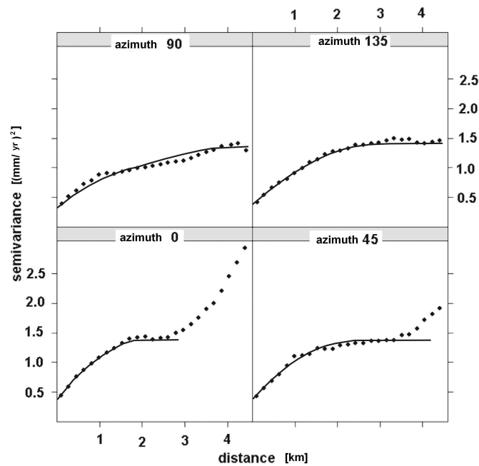
Fig. 4.7. Directional semivariograms for downthrown block of the Bedzinski fault
