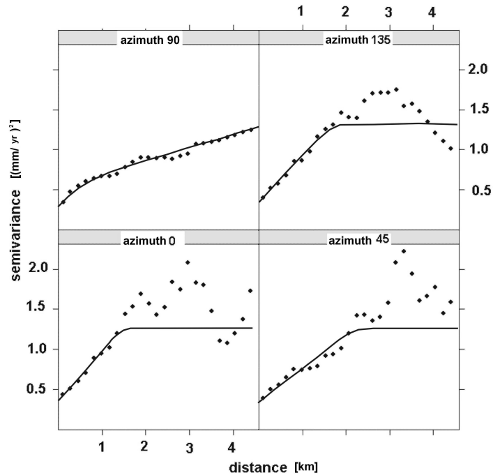
Fig. 4.8. Directional semivariograms for upthrown block of Bedzinski fault
