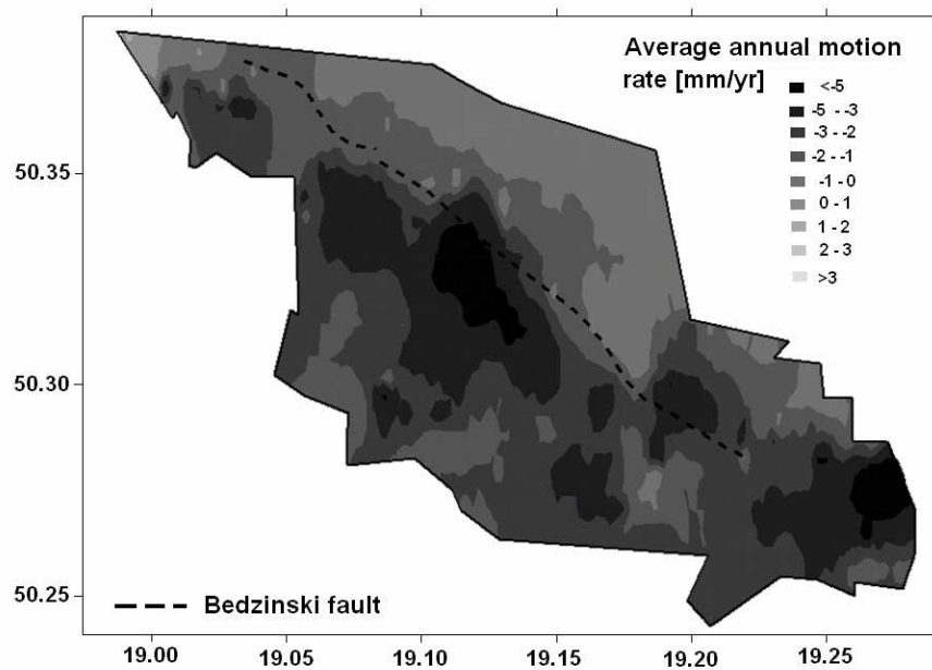
Fig.4.1. Values of average annual motion rates estimated using inverse distance interpolation method
