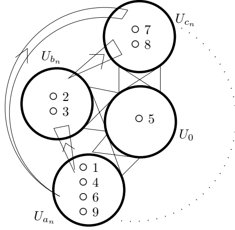
Fig. 2. The sequence 1,2,3,4,5,6,7,8,9 realises the fragment ‘... a, b, b, a, 0, a, c, c, a... ’ of \mathcal{C}_n .
