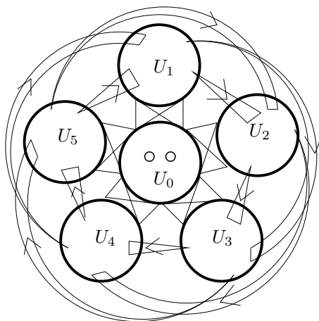
Fig. 1. A hypergraph from the family \mathcal{J}(2, 5) .
