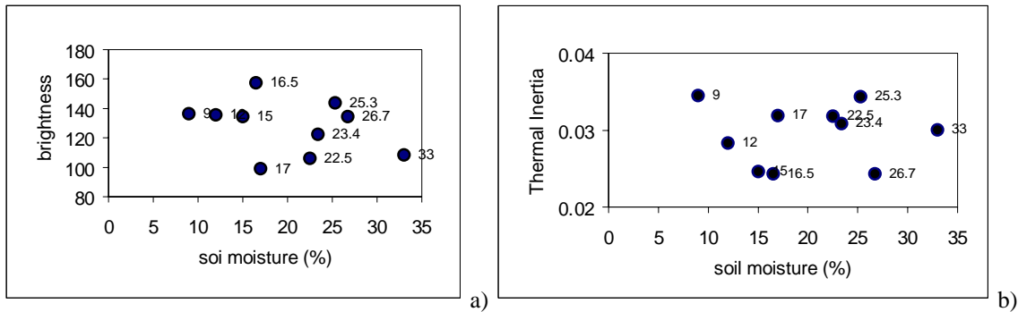
Figure 13 Correlation between brightness a) and thermal inertia b) and soil moisture for test fields.
