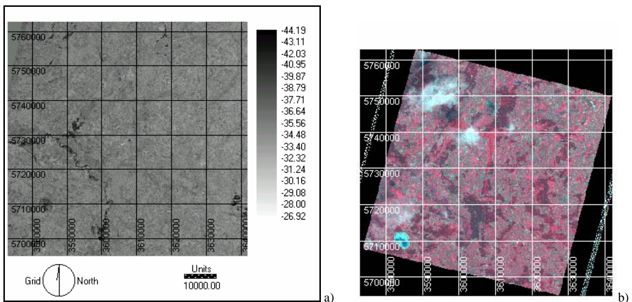
Figure 1. Study area, a) Radar image – ERS2, b) False Color Composition of LANDSAT TM234.
