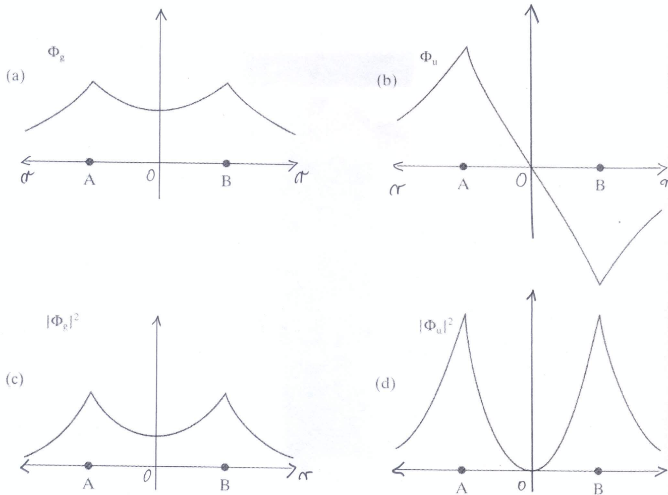
Figure 10.9 Wave functions \Phi_g and \Phi_u ((a) and (b)) and electron probability densities |\Phi_g|^2 , |\Phi_u|^2 ((c) and (d)) for the hydrogen molecular ion H_2^+ , plotted along the internuclear line to an arbitrary scale. The points A and B represent the positions of the two protons.
