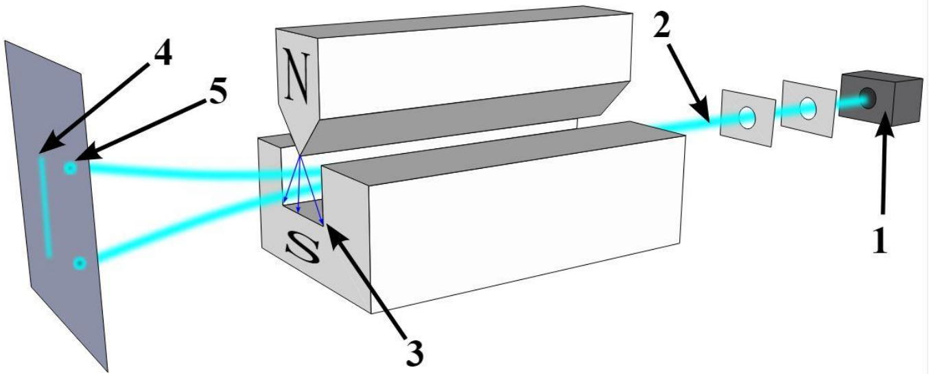
Stern–Gerlach experiment: Silver atoms travelling through an inhomogeneous magnetic field, and being deflected up or down depending on their spin; (1) furnace, (2) beam of silver atoms, (3) inhomogeneous magnetic field, (4) classically expected result, (5) observed result
