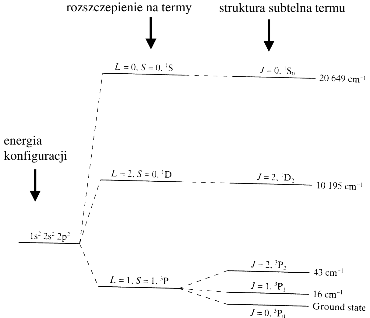
Figure 8.8 The splitting of the ground state configuration of carbon.
