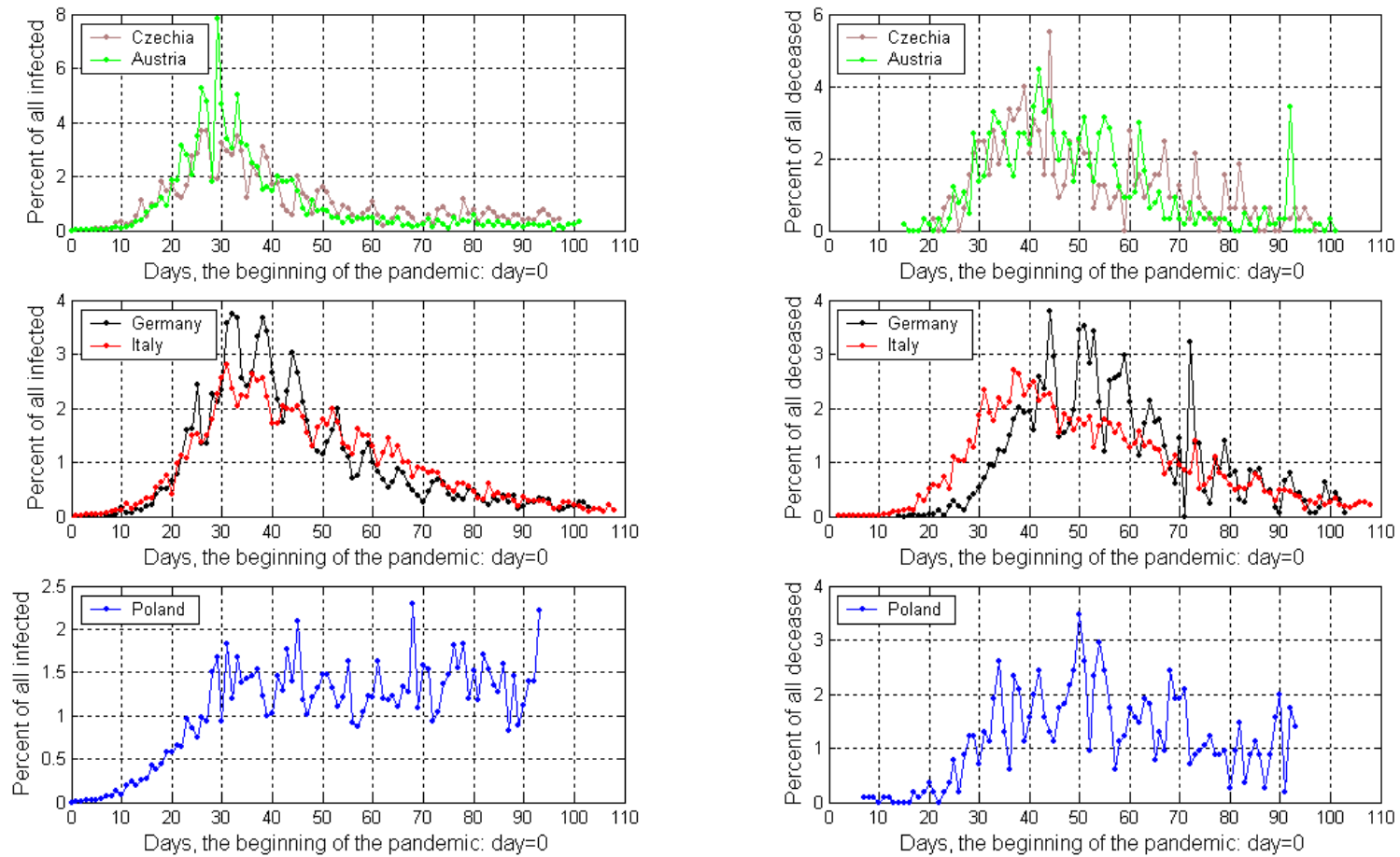
Fig. 4. Comparison: selected countries in groups, on the left – persons infected daily, on the right – persons deceased daily. 100% means all infected/deceased in each country until yestarday. Day=0 represents the beginning of the pandemic – may be different for each country, and only for the USA the graphs have been shifted horizontally by additional 14 days, to emphasize the matching shape.
