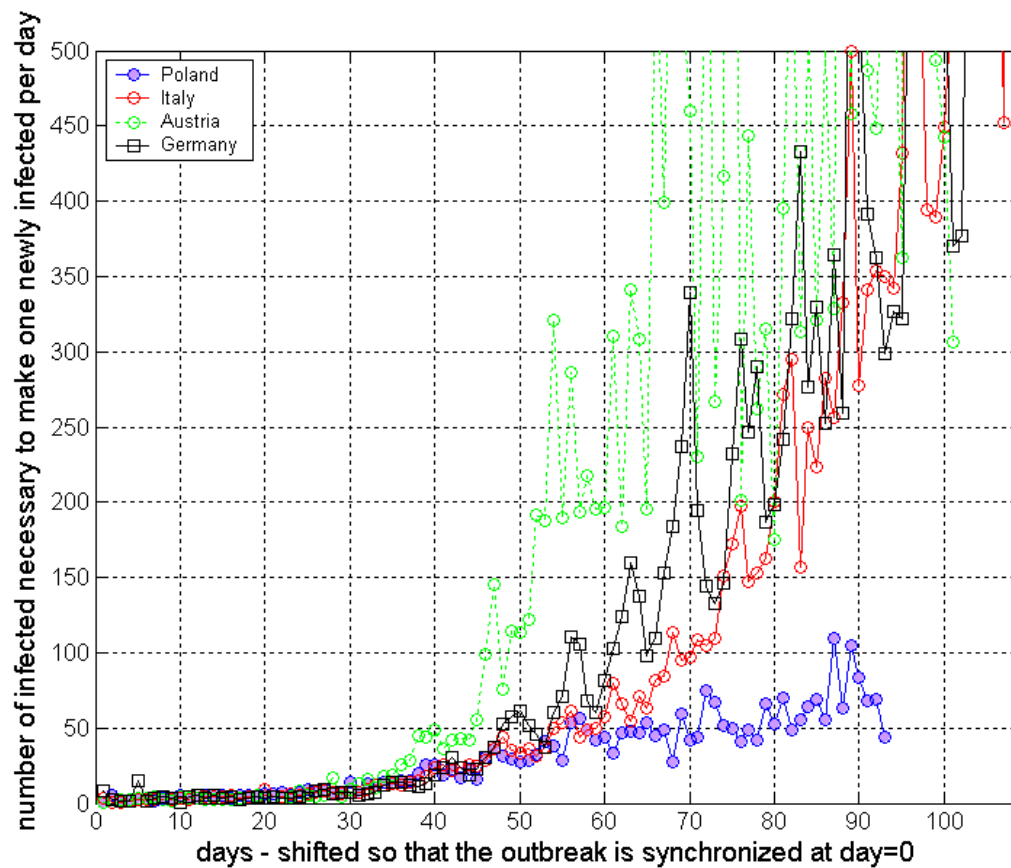
Fig. 3. The statistically average number of already infected persons, p (see Tab. 1), necessary to produce one newly infected person per day (calculated a posteriori). Note that the cured ones have not been subtracted from the total number of infected, therefore this parameter provides only the alternative way to interpret graphs in Fig. 2. The higher is the p parameter, the slower the number of infected grows (in the logarithmic scale!). For example, p=10 means that during given day the number of infected persons increased from 10 to 11 (on the average) or from 2000 to 2200, or from 15000 to 16500, etc.
