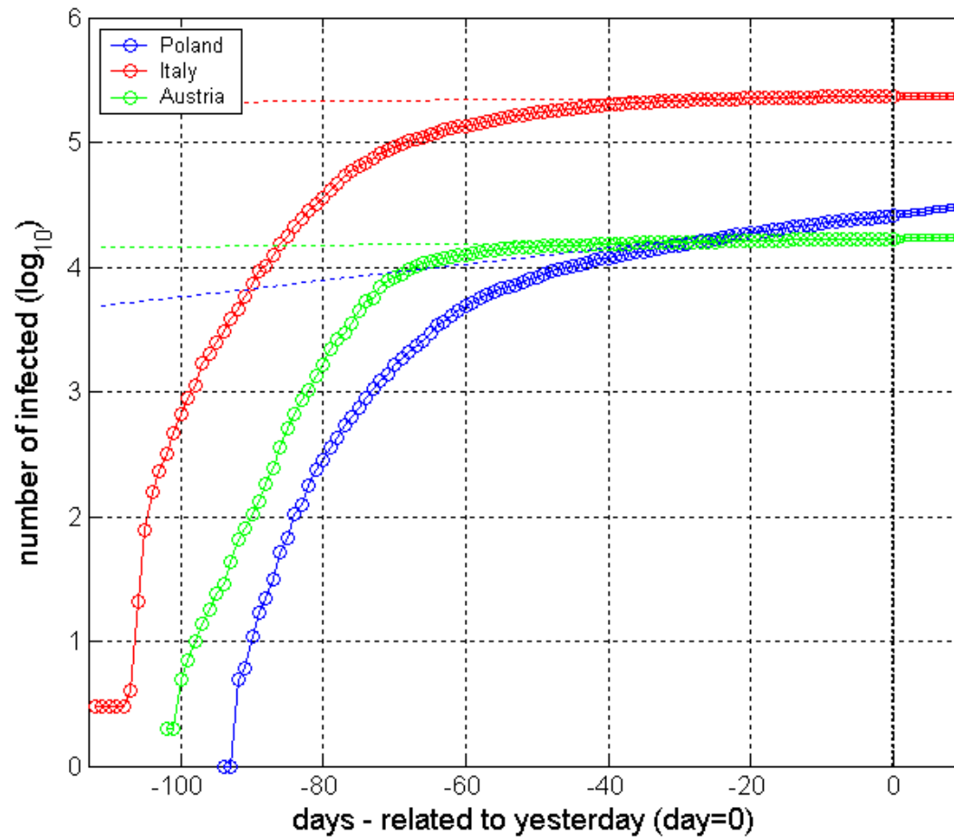
Fig. 1. Total number of infected persons. The straight lines provide reference to the “logarithmically constant” growing rate: red-dotted ( r=843/842 ), green-dotted ( r=661/660 ), blue-dotted ( r=67/66 ), when y(n+1)=y(n) \cdot r and n denotes the day number. Square markers with the same color show the predicted data – see Tab. 2.
