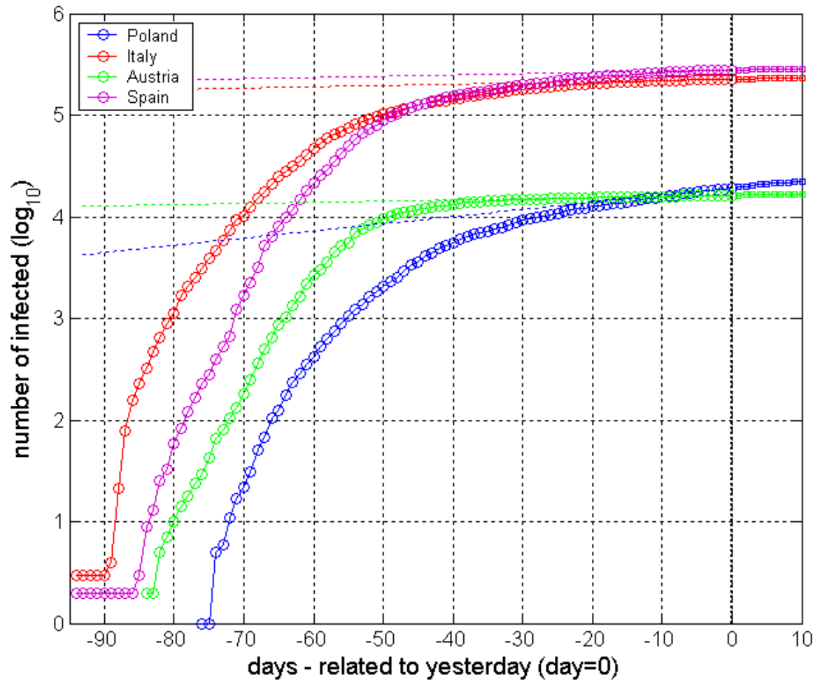
Fig. 1. Total number of infected persons. The straight lines provide reference to the “logarithmically constant” growing rate: red-dotted ( r=343/342 ), magenta-dotted ( r=351/350 ), green-dotted ( r=372/371 ), blue-dotted ( r=62/61 ), when y(n+1)=y(n) \cdot r and n denotes the day number. Square markers with the same color show the predicted data – see Tab. 2.
