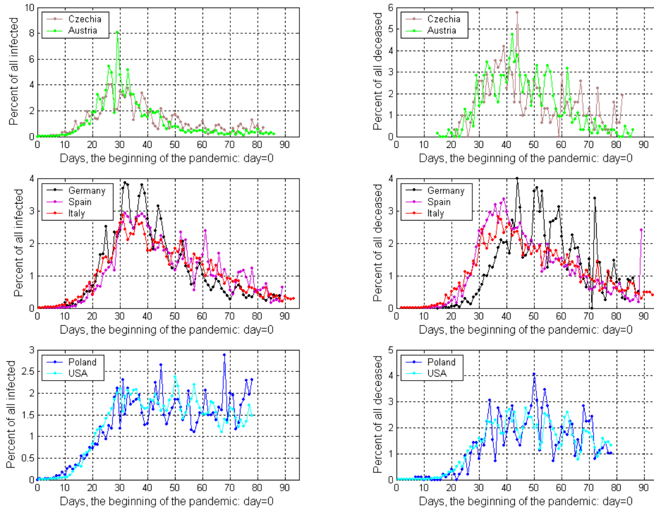
Fig. 4. Comparison: selected countries in groups, on the left – persons infected daily, on the right – persons deceased daily. 100% means all infected/deceased in each country until yestarday. Day=0 represents the beginning of the pandemic – may be different for each country, and only for the USA the graphs have been shifted horizontally by additional 14 days, to emphasize the matching shape.
