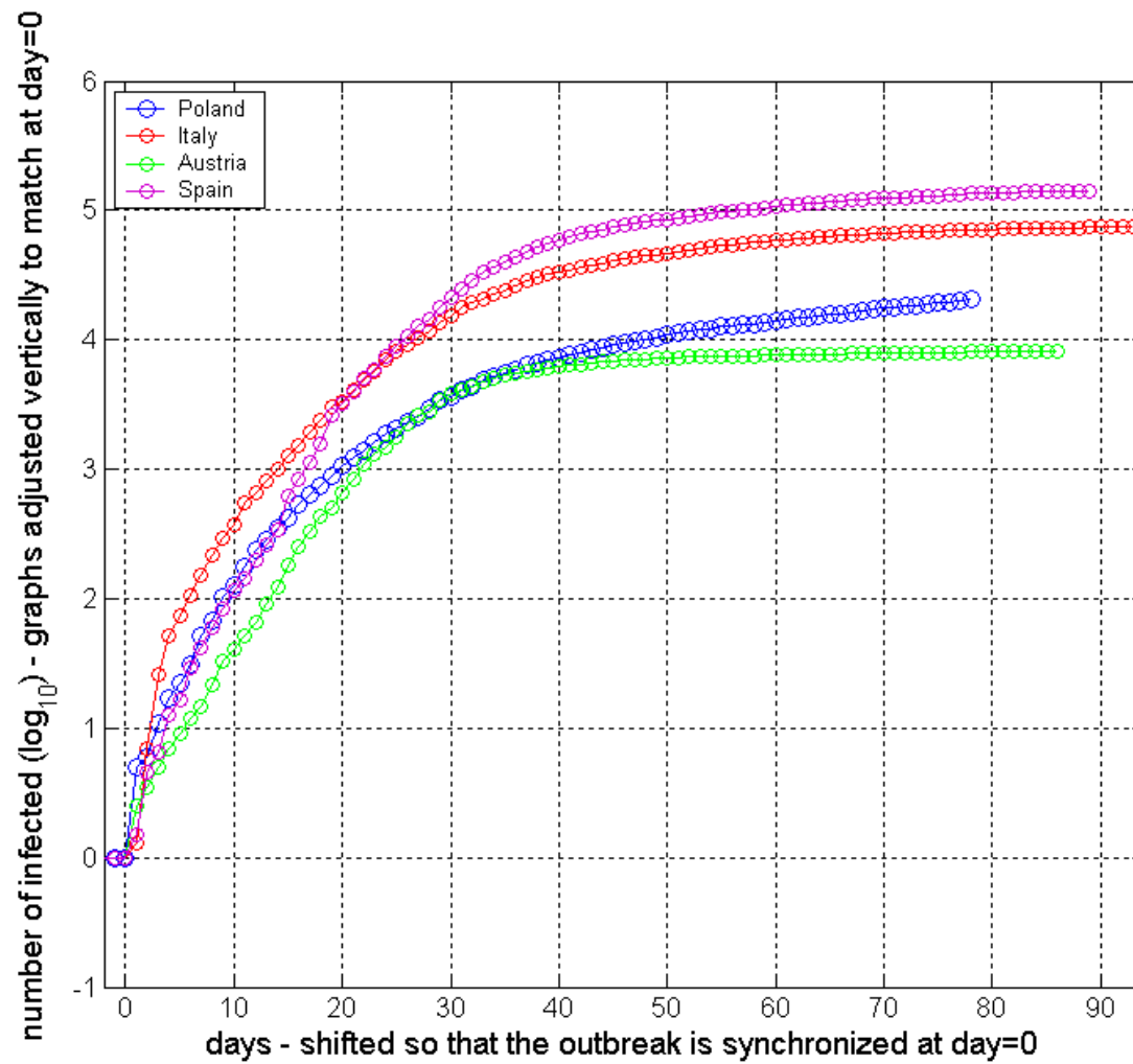
Fig. 2. The same graphs as in Fig. 1, but the curves have been shifted, both vertically and horizontally, to make it possible to visually compare the evolution of the pandemic in the selected countries. The comparison may suggest some anticipation of the future evolution for each country. The flat ending of the curve running horizontally would mean there are no newly infected persons reported.
