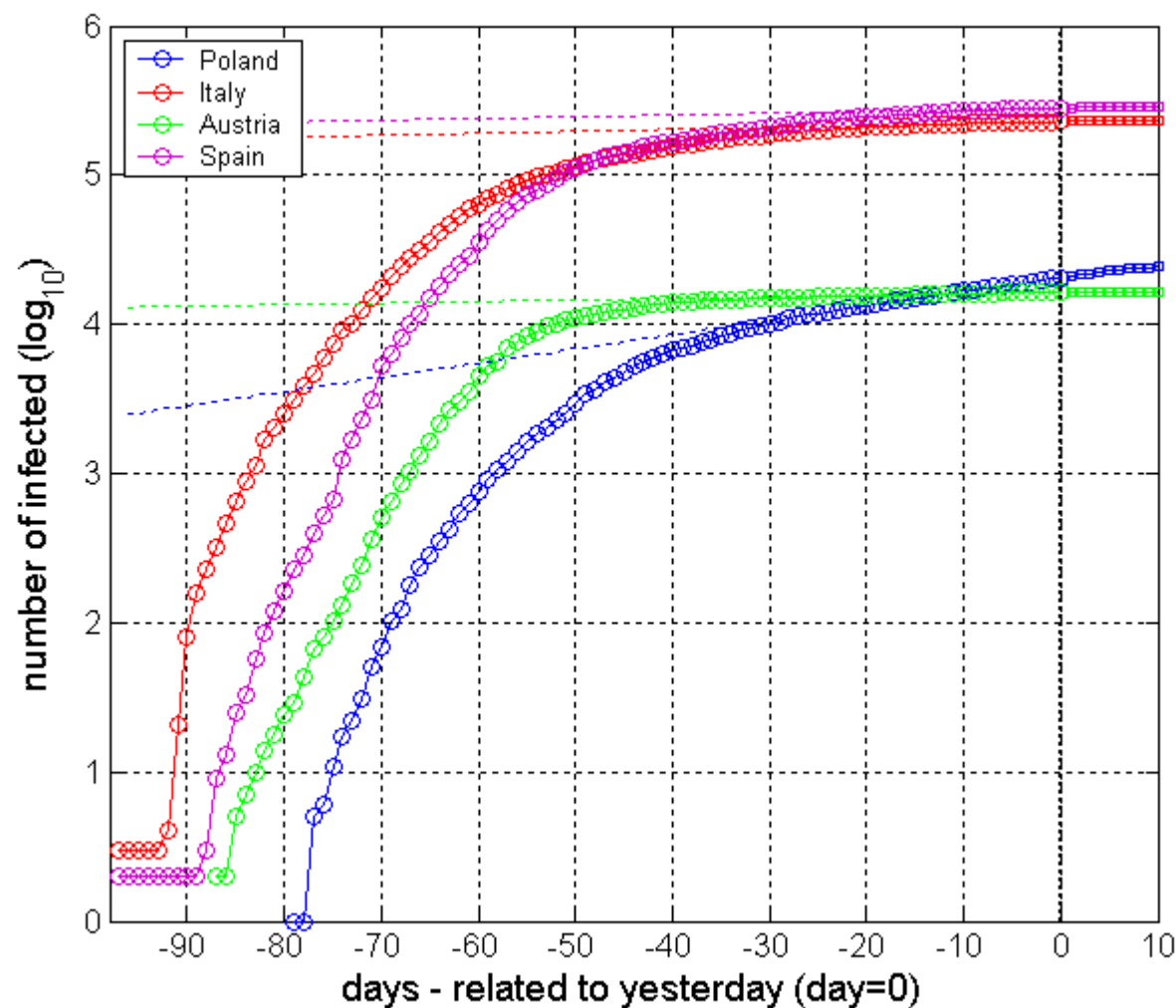
Fig. 1. Total number of infected persons. The straight lines provide reference to the “logarithmically constant” growing rate: red-dotted ( r=332/331 ), magenta-dotted ( r=368/367 ), green-dotted ( r=415/414 ), blue-dotted ( r=46/45 ), when y(n+1)=y(n) \cdot r and n denotes the day number. Square markers with the same color show the predicted data – see Tab. 2.
