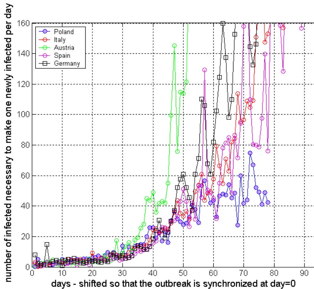
Fig. 3. The statistically average number of already infected persons, p (see Tab. 1), necessary to produce one newly infected person per day (calculated a posteriori). Note that the cured ones have not been subtracted from the total number of infected, therefore this parameter provides only the alternative way to interpret graphs in Fig. 2. The higher is the p parameter, the slower the number of infected grows (in the logarithmic scale!). For example, p=10 means that during given day the number of infected persons increased from 10 to 11 (on the average) or from 2000 to 2200, or from 15000 to 16500, etc.
