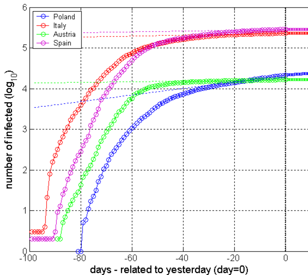
Fig. 1. Total number of infected persons. The straight lines provide reference to the “logarithmically constant” growing rate: red-dotted ( r=370/369 ), magenta-dotted ( r=456/455 ), green-dotted ( r=534/533 ), blue-dotted ( r=54/53 ), when y(n+1)=y(n) \cdot r and n denotes the day number. Square markers with the same color show the predicted data – see Tab. 2.
