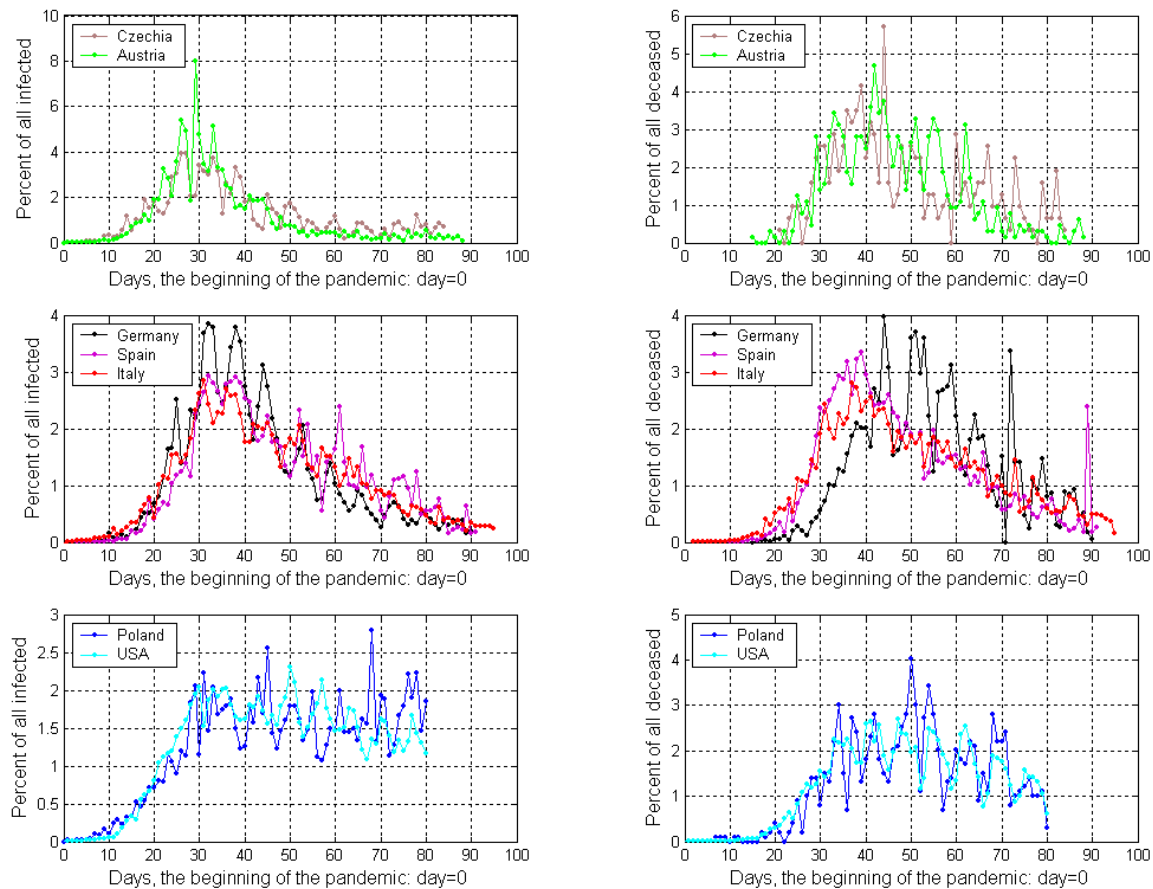
Fig. 4. Comparison: selected countries in groups, on the left – persons infected daily, on the right – persons deceased daily. 100% means all infected/deceased in each country until yesterday. Day=0 represents the beginning of the pandemic – may be different for each country, and only for the USA the graphs have been shifted horizontally by additional 14 days, to emphasize the matching shape.
