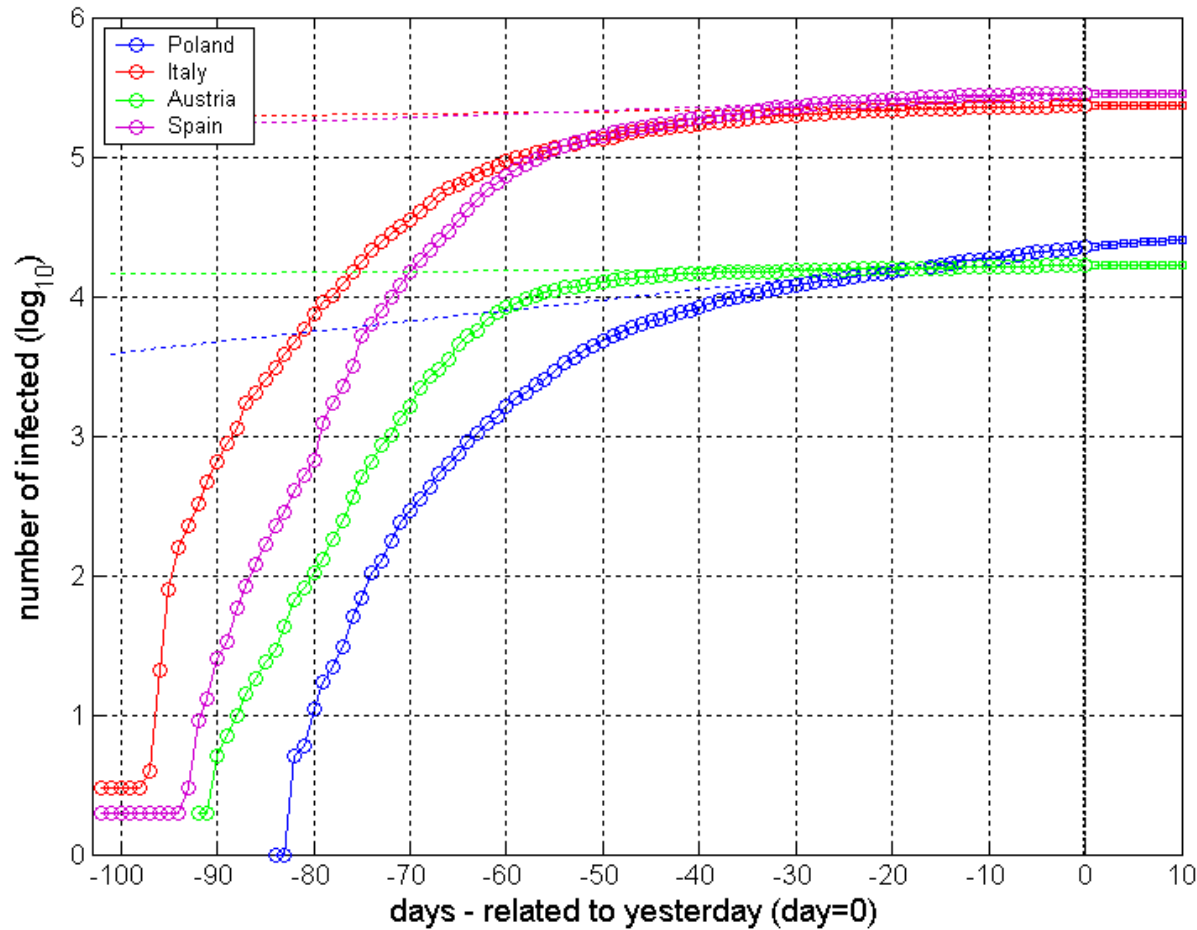
Fig. 1. Total number of infected persons. The straight lines provide reference to the “logarithmically constant” growing rate: red-dotted ( r=544/543 ), magenta-dotted ( r=178/177 ), green-dotted ( r=709/708 ), blue-dotted ( r=58/57 ), when y(n+1)=y(n) \cdot r and n denotes the day number. Square markers with the same color show the predicted data – see Tab. 2.
