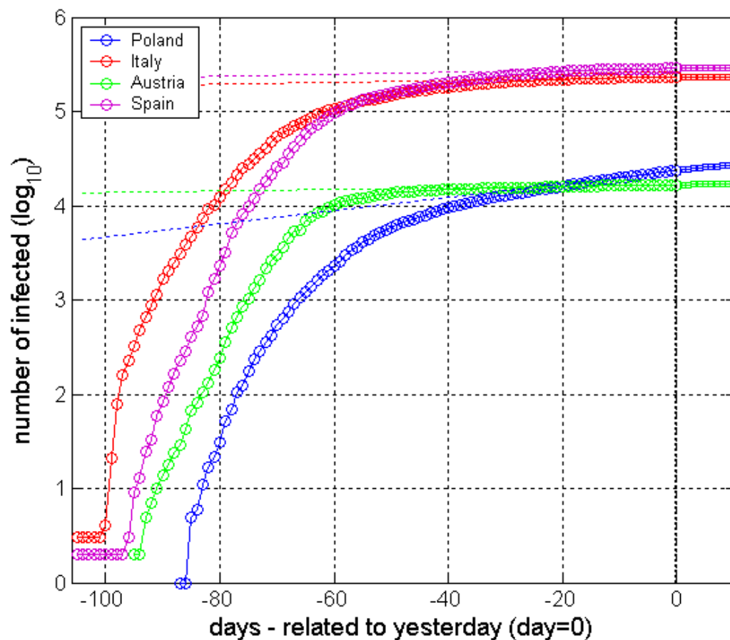
Fig. 1. Total number of infected persons. The straight lines provide reference to the “logarithmically constant” growing rate: red-dotted ( r=449/448 ), magenta-dotted ( r=418/417 ), green-dotted ( r=528/527 ), blue-dotted ( r=62/61 ), when y(n+1)=y(n) \cdot r and n denotes the day number. Square markers with the same color show the predicted data – see Tab. 2.
