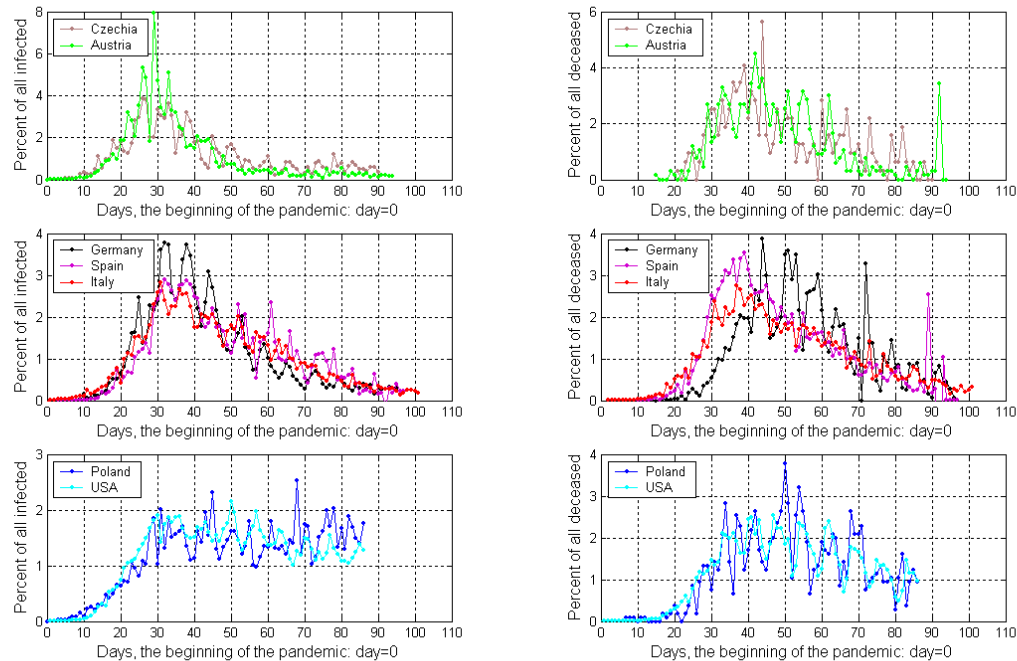
Fig. 4. Comparison: selected countries in groups, on the left – persons infected daily, on the right – persons deceased daily. 100% means all infected/deceased in each country until yestarday. Day=0 represents the beginning of the pandemic – may be different for each country, and only for the USA the graphs have been shifted horizontally by additional 14 days, to emphasize the matching shape.
