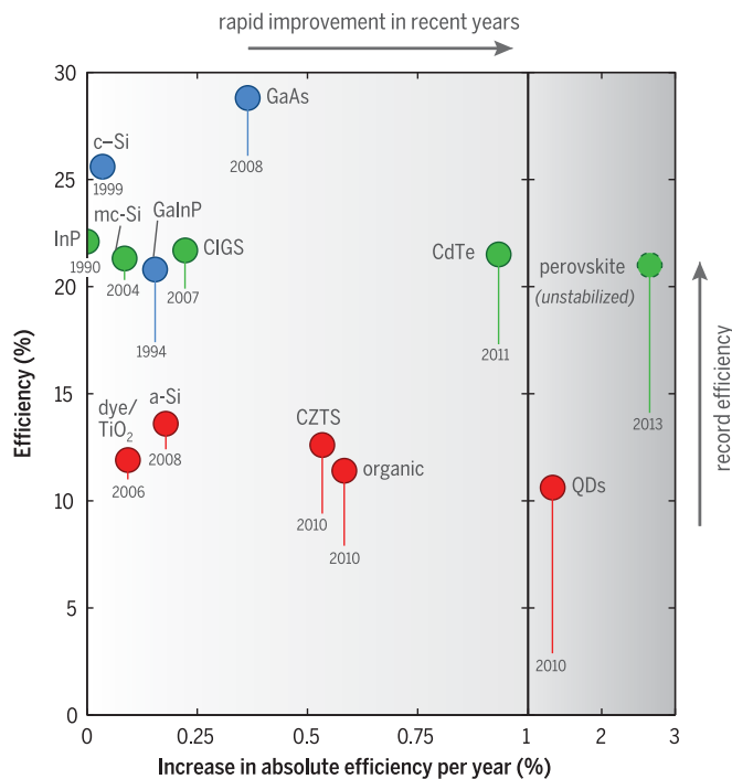
Fig. 5. Rates of improvement in solar cell efficiency over recent years. Average improvements were
