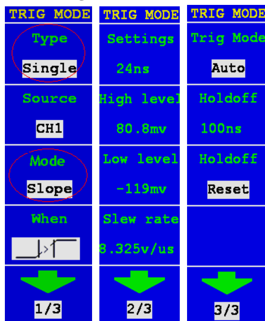
Fig. 5-22 Slope Trigger menu
