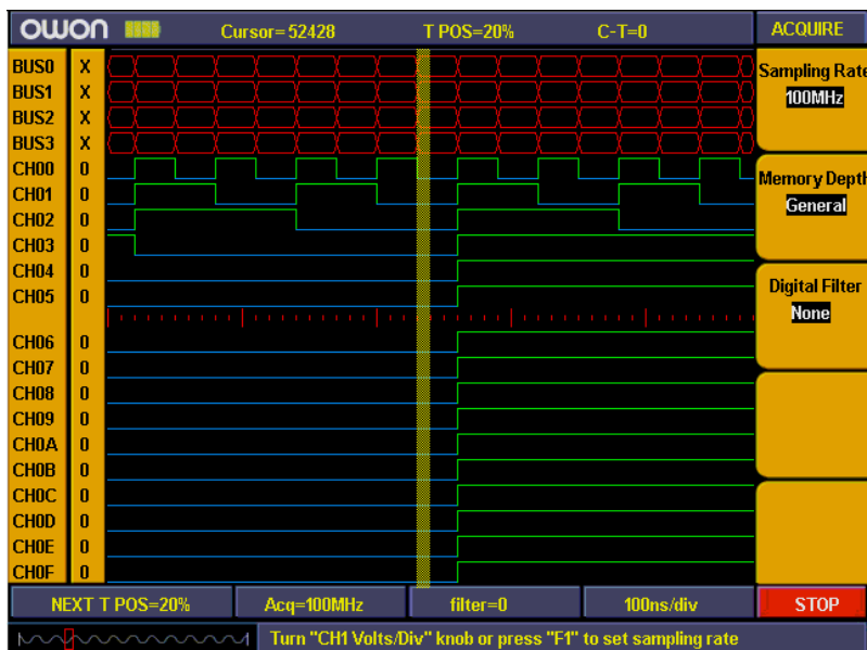
Fig. 5-53: Sampling setting
