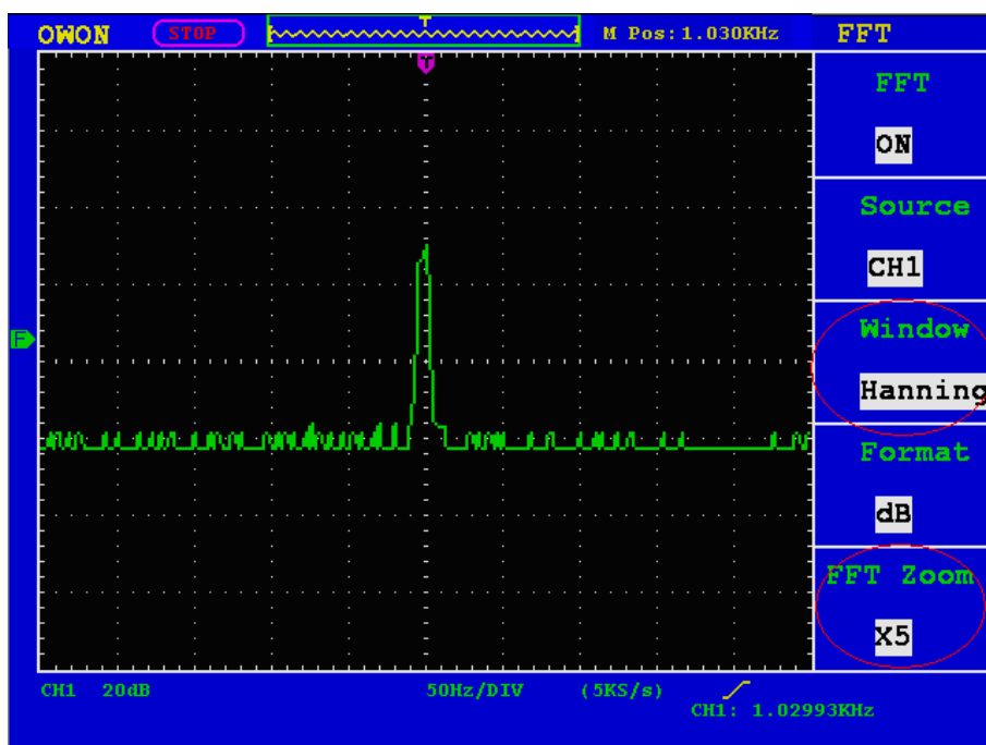
Fig.5-12 Hanning window
