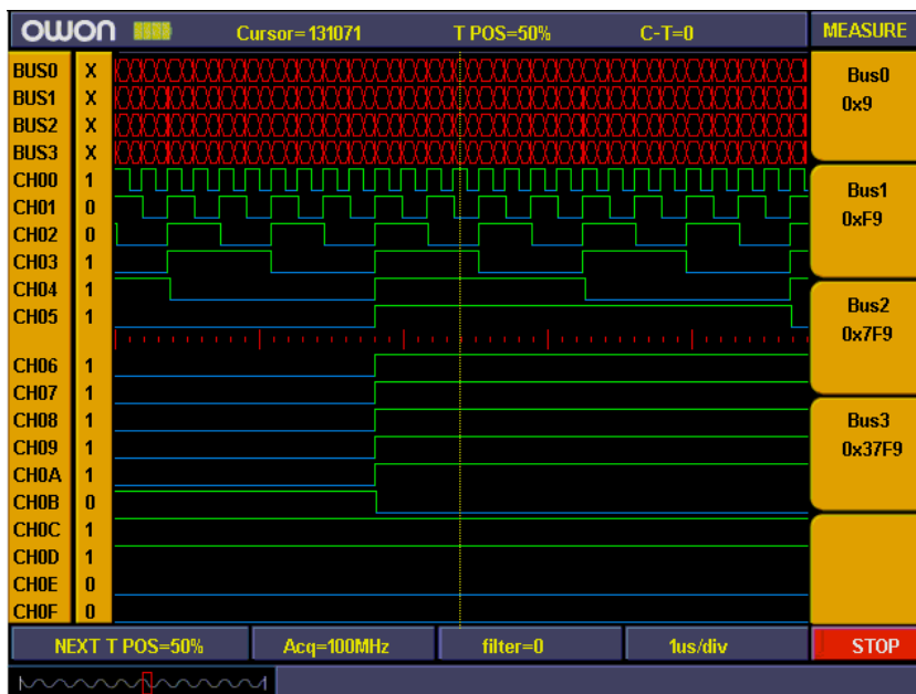
Fig.5-72: Bus measurement
