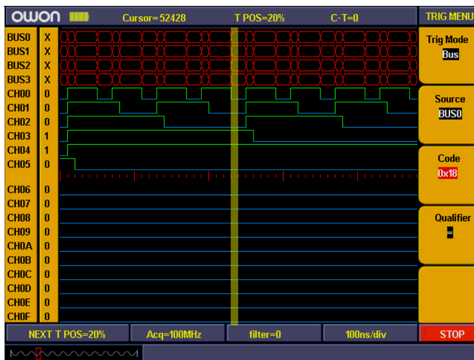
Fig.5-57: Bus trigger
