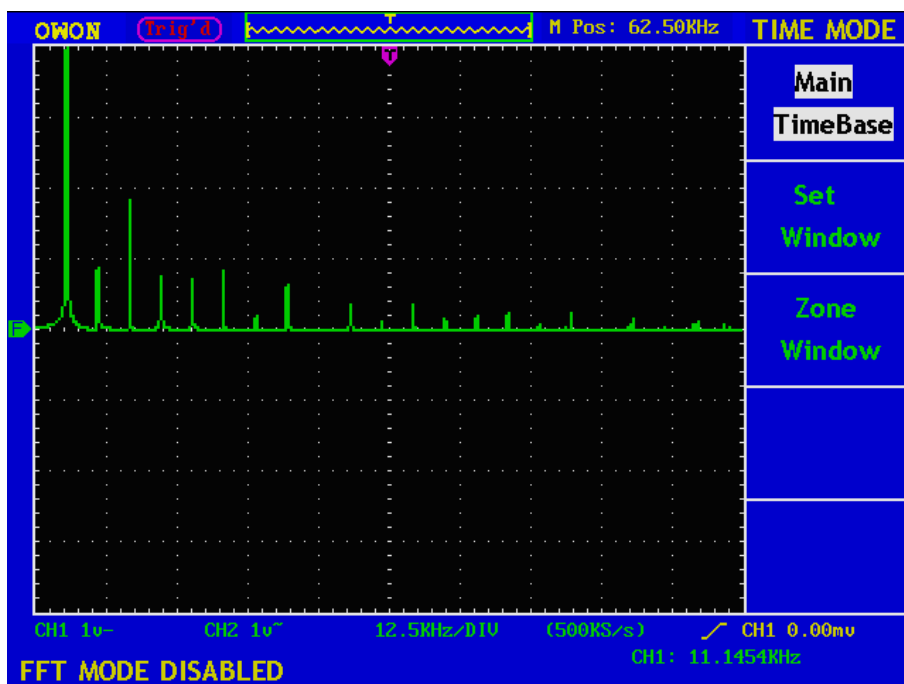
Fig.5-17 Set Window disable under FFT mode
