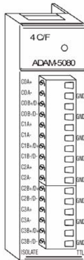
Figure 52: ADAM-5080 Module
