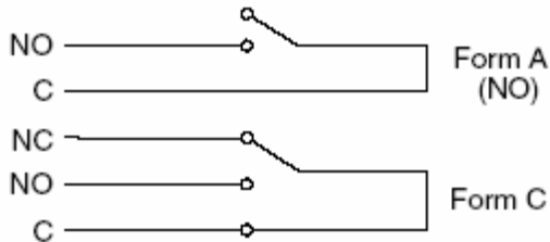
Figure 48: Relay output
