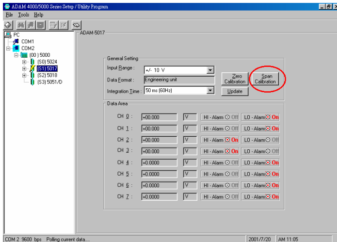
Figure 24: Span calibration
