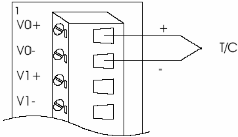
Figure 19: Thermocouple input
