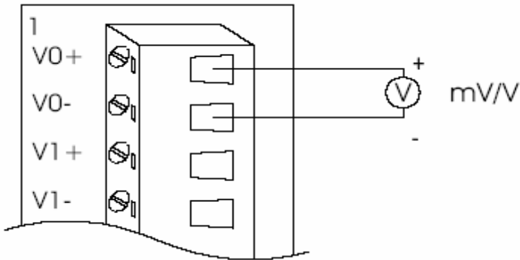
Figure 8: Millivolt and volt input
