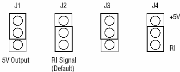
Figure 68: Jumper Settings
