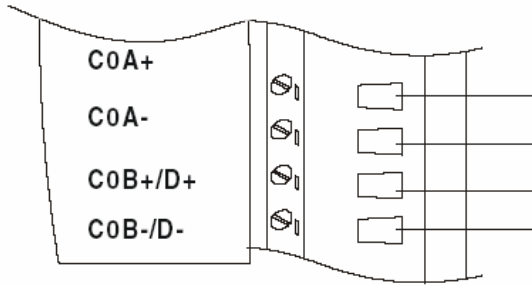
Figure 56: Wiring for Up/Down Counting
