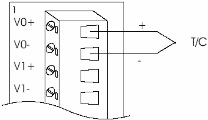
Figure 17: Thermocouple input
