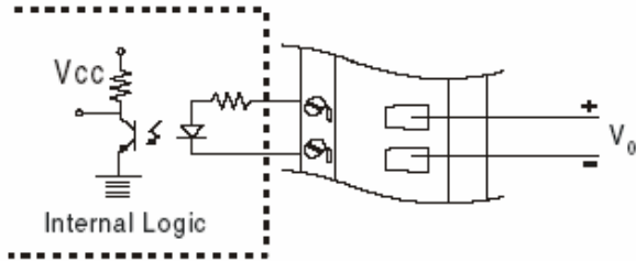
Figure 53: Isolated Input Level
