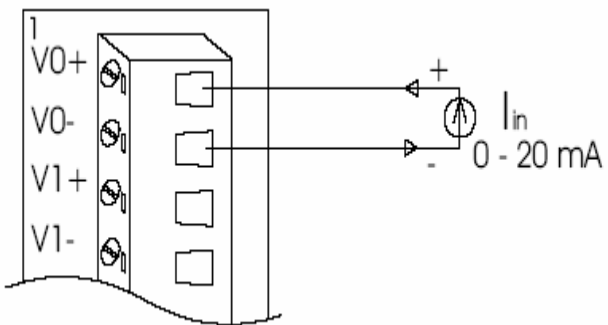
Figure 13: Process current input
