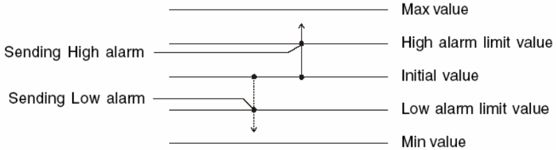
Figure 60: Sending Alarm Signal (recommended settings)
