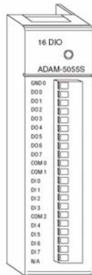
Figure 39: ADAM-5055S module front view
