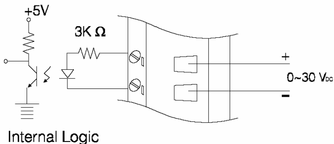
Figure 38: Isolation digital input (ADAM-5052)
