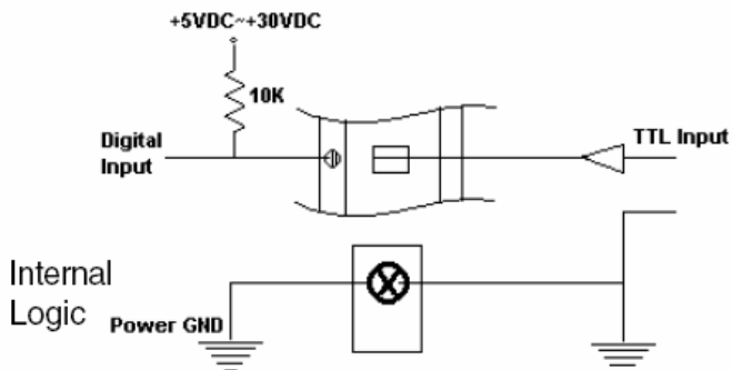
Figure 33: TTL input (ADAM-5051/5051D)
