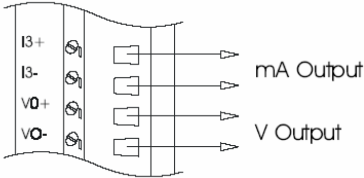
Figure 21: Analog output
