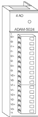
Figure20: ADAM-5024 module frontal view
