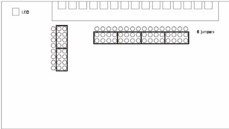
Figure 63: Jumper Location on the ADAM-5081 Module
