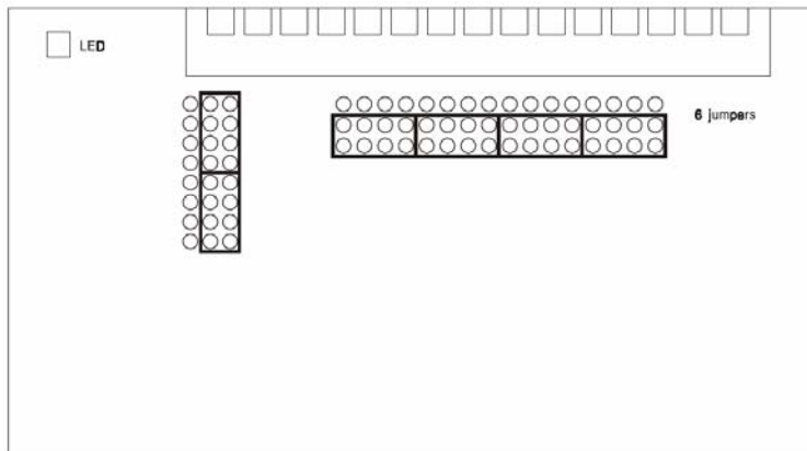
Figure 63: Jumper Location on the ADAM-5080 Module
