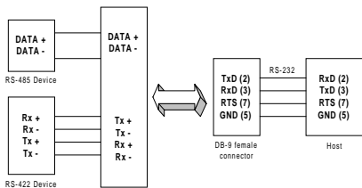
ADAM-4520 Converter Connection Diagram
