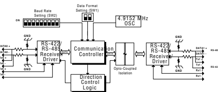
ADAM-4510 Repeater Function Diagram
