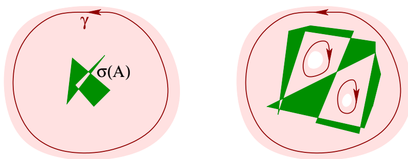
Figure 5.2.1. A cycle encircling the spectrum.
